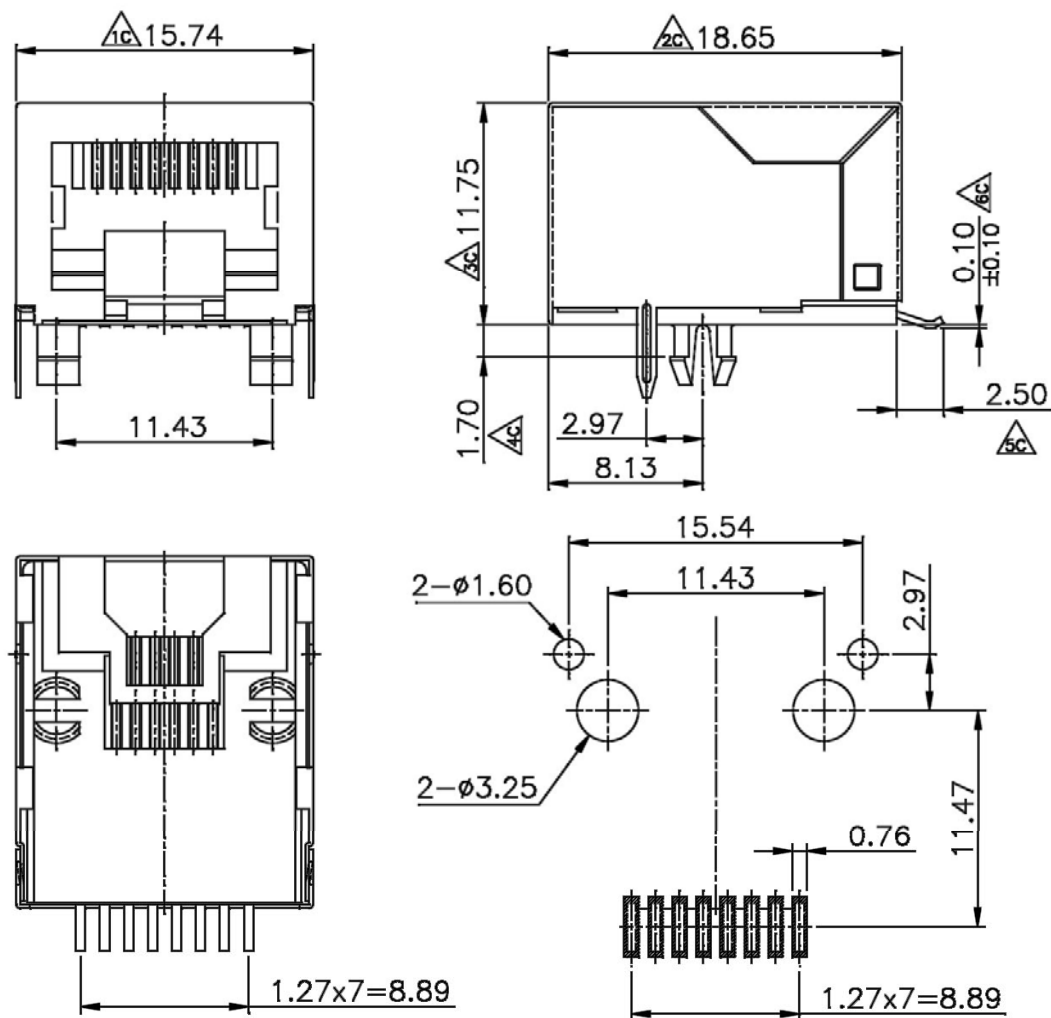
PCB LAYOUT/TOP VIEW
